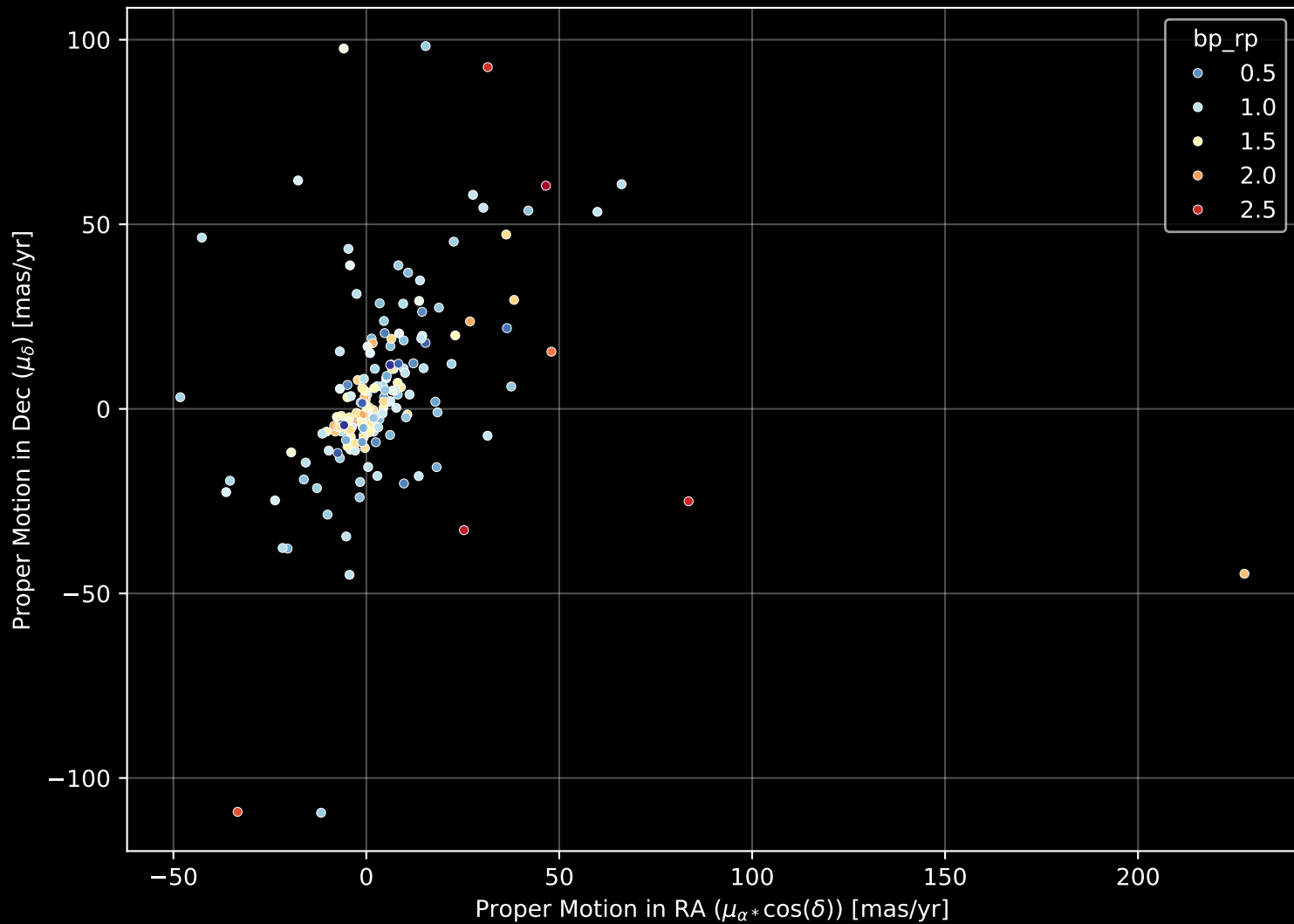
APOGEE DR17 Field: [CVZ_OB20_btx] Proper Motion Diagram (n= 185)
