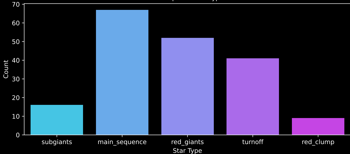
APOGEE DR17 Field: [CVZ_OB20_btx] Count plot of Star Type
