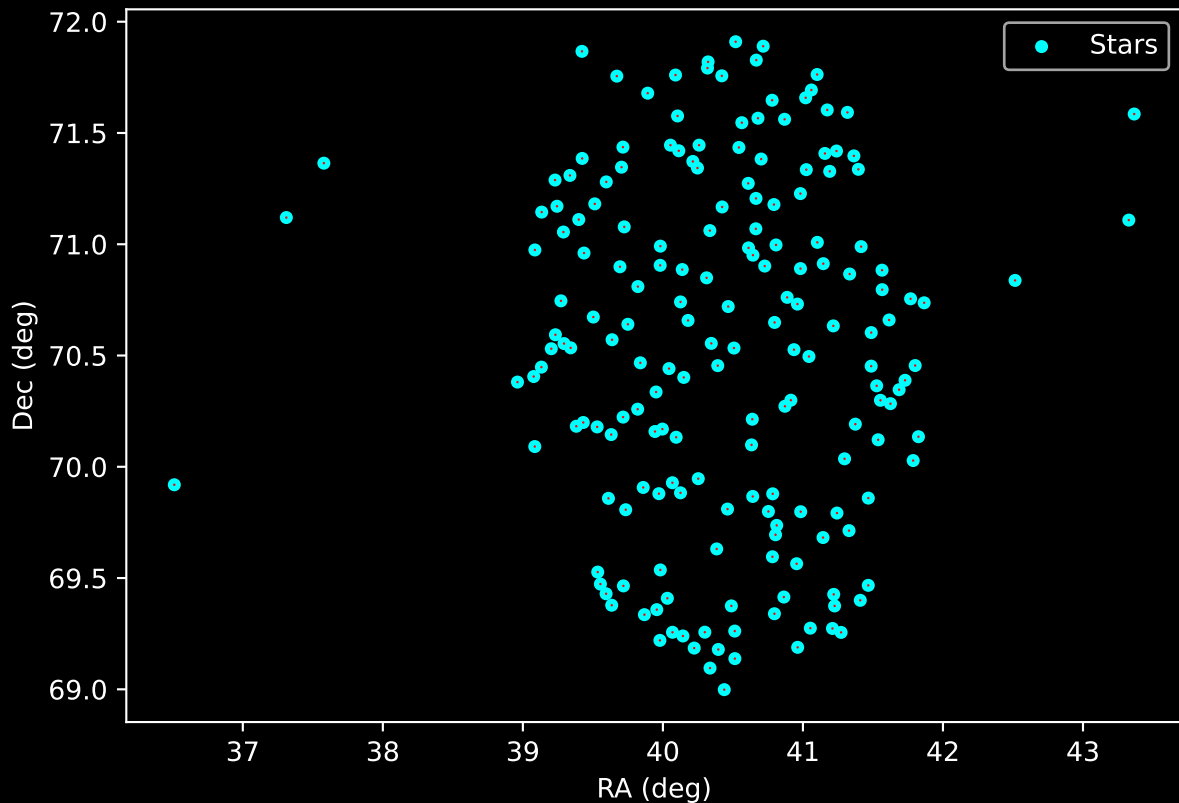
APOGEE DR17 Field: [CVZ_OB20_btx] Proper Motion Vectors for Gaia Star Field (n= 185)
