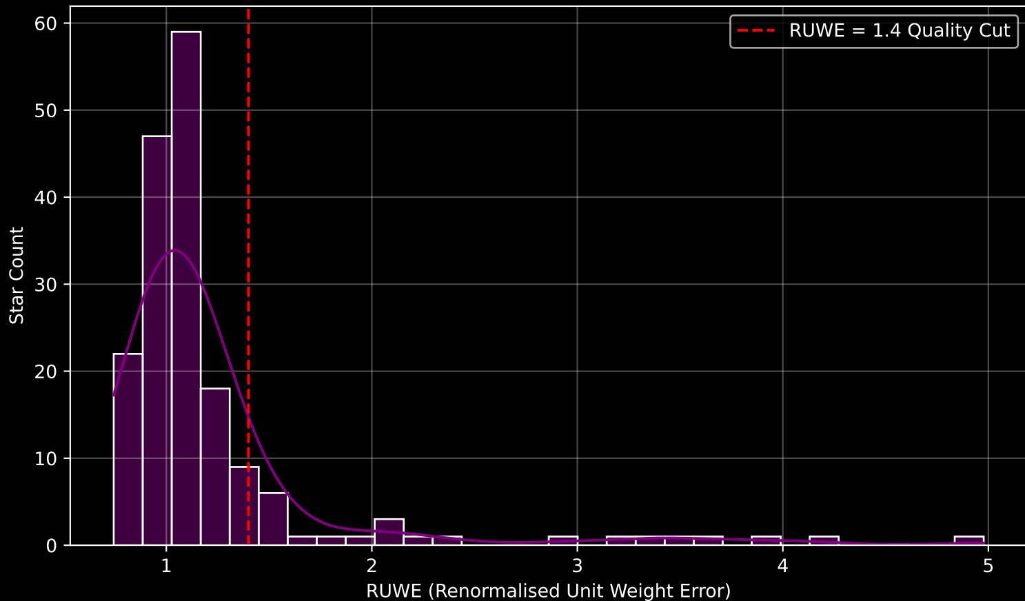
GAPOGEE DR17 Field [CVZ_OB20_btx] RUWE Distribution (n= 177)
