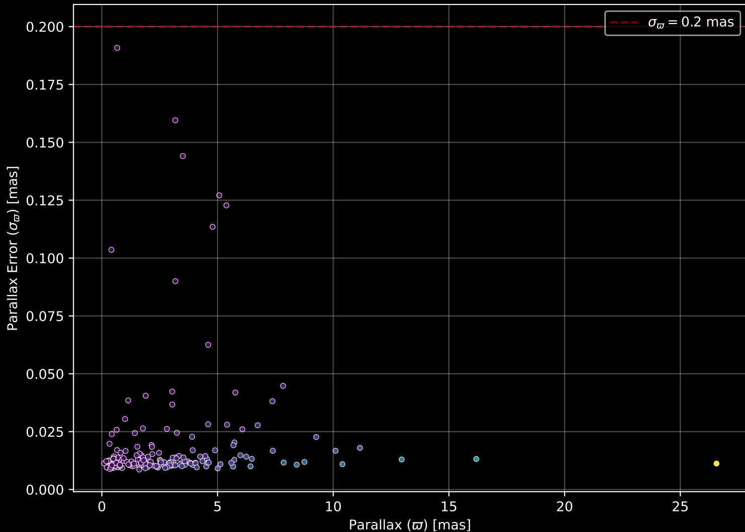
APOGEE DR17 Field: [CVZ_OB20_btx] Parallax Quality (n= 185)
