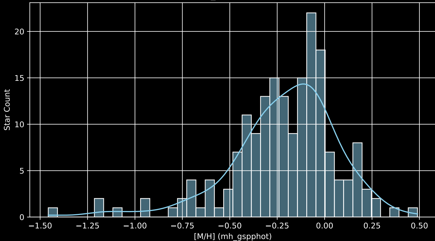
APOGEE DR17 Field: [CVZ_OB20_btx [M/H] (mh_gspphot) (n= 184)
