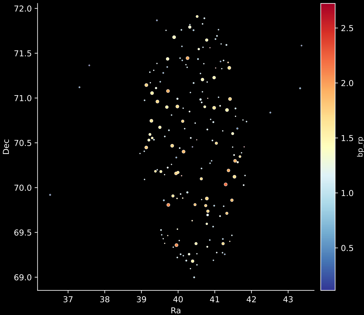
APOGEE DR17 Field: [CVZ_OB20_btx] Stars: 185
